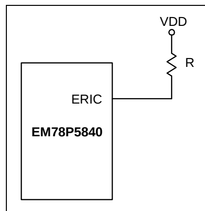
Figure 7-11a ERIC Mode Application Circuit
