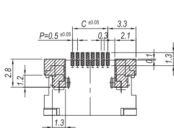
PCB LAYOUT (05002HR-00A01)
