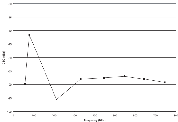
Figure 24: CSO vs. Frequency
