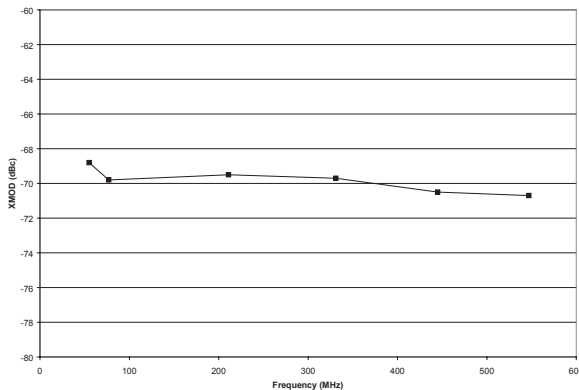
Figure 22: XMOD vs. Frequency
