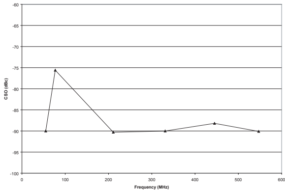
Figure 21: CSO vs. Frequency
