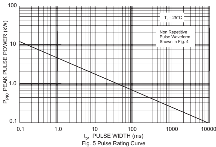
Fig. 5 Pulse Rating Curve
