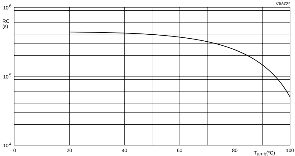
Fig.14 RC product as a function of ambient free air temperature: typical curve.
