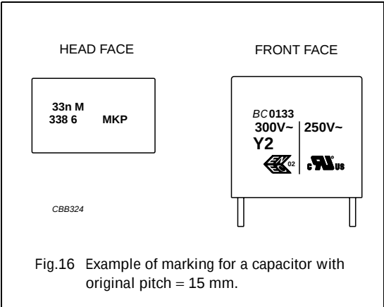
Fig.15 Example of marking for a capacitor with original pitch = 7.5 and 10 mm.
