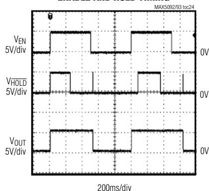
ENABLE AND HOLD TIMING
