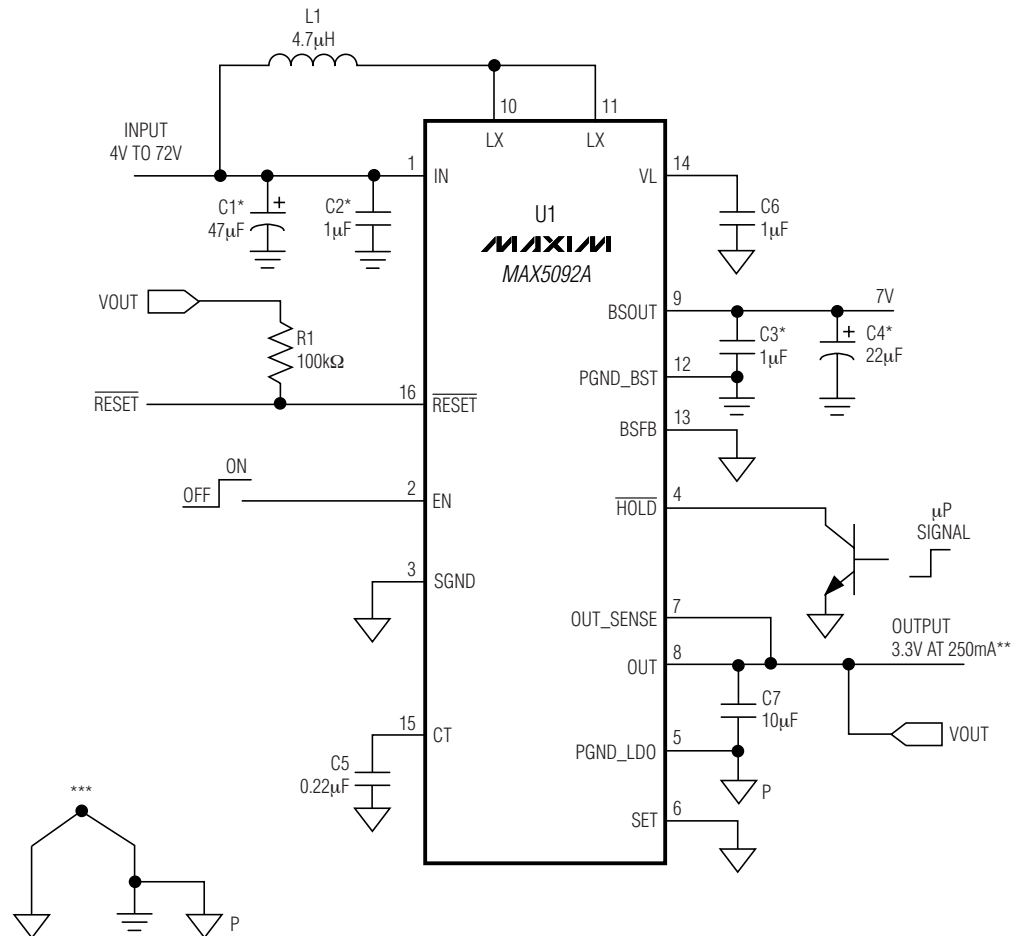
Figure 4. MAX5092A Typical Application Circuit with Factory Preprogrammed LDO and Boost Output Voltages
