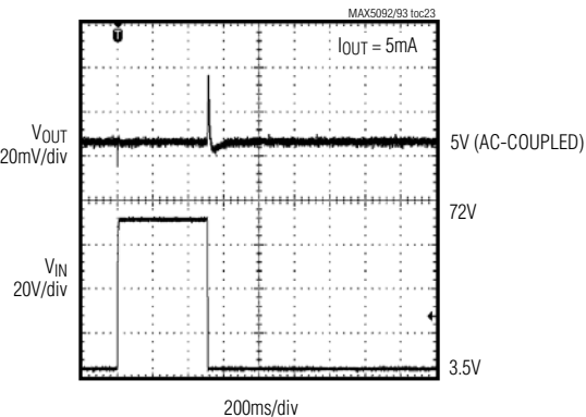
INPUT-VOLTAGE STEP RESPONSE
