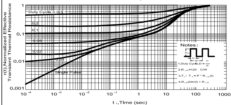
Transient Thermal Response Curve
