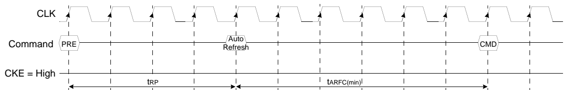
Figure 65.11 Auto Refresh
