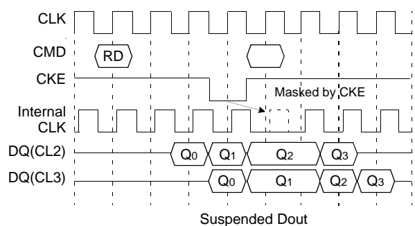
Figure 65.1 Clock Suspend
