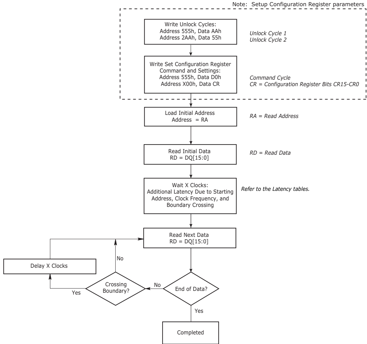
Figure 12.2. Synchronous Read
