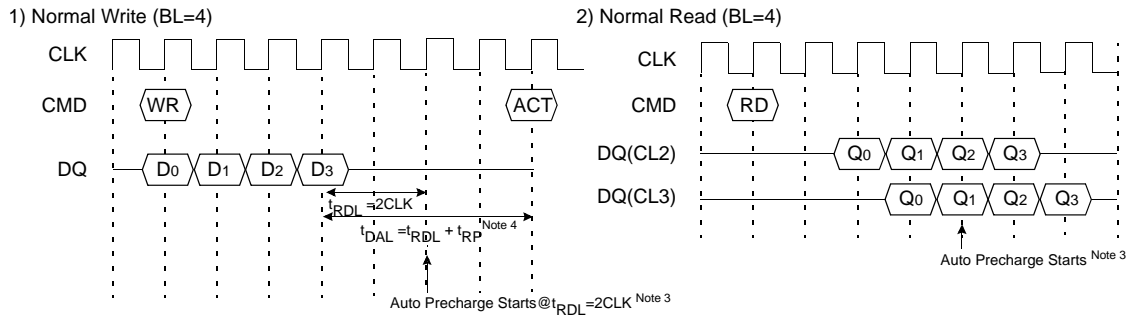
Figure 65.7 Auto Precharge
