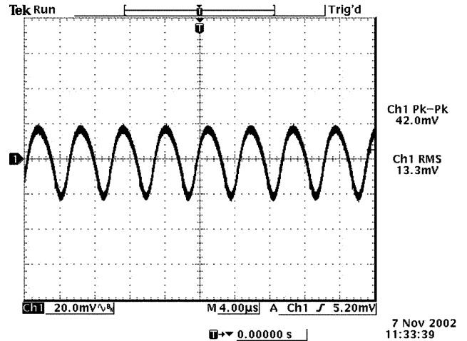
Ripple and noise at full load and 12Vdc input, 3.3Vdc output, full load with an external 22µF tantalum capacitor and Ta=25° C
