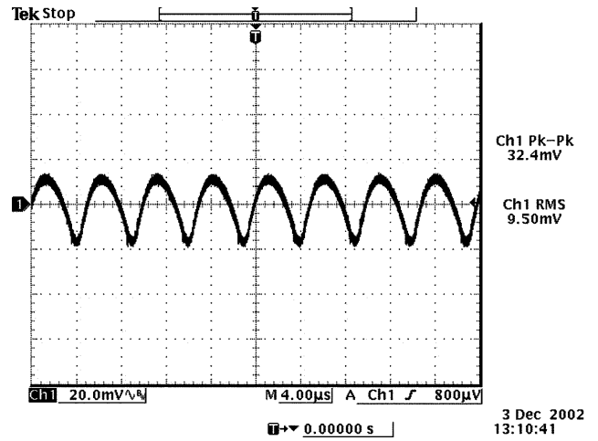
Ripple and noise at full load and 12Vdc input, 2.0Vdc output, full load with an external 22µF tantalum capacitor and Ta=25° C
