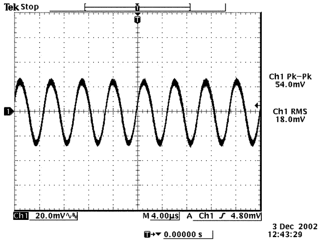
Ripple and noise at full load and 12Vdc input, 5.0Vdc output, full load with an external 22µF tantalum capacitor and Ta=25° C
