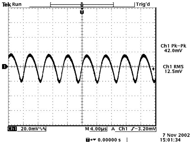
Ripple and noise at full load and 12Vdc input, 2.5Vdc output, full load with an external 22µF tantalum capacitor and Ta=25° C
