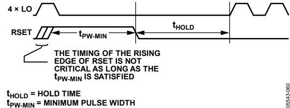
Figure 58. Timing of the RSET Signal to 4 LO
