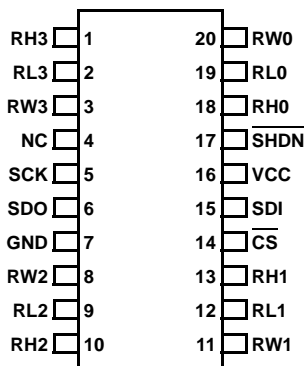
ISL22446 (20 LD TSSOP) TOP VIEW
