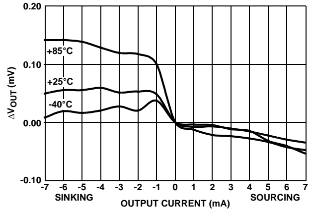
FIGURE 77. LOAD REGULATION
