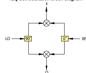
I&Q demodulation block diagram
