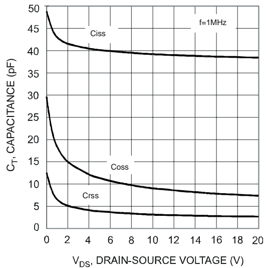
Fig. 10 Typical Capacitance
