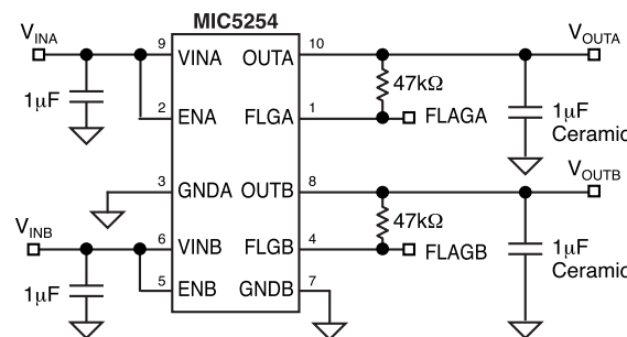
Dual Output LDO with Error Flags
