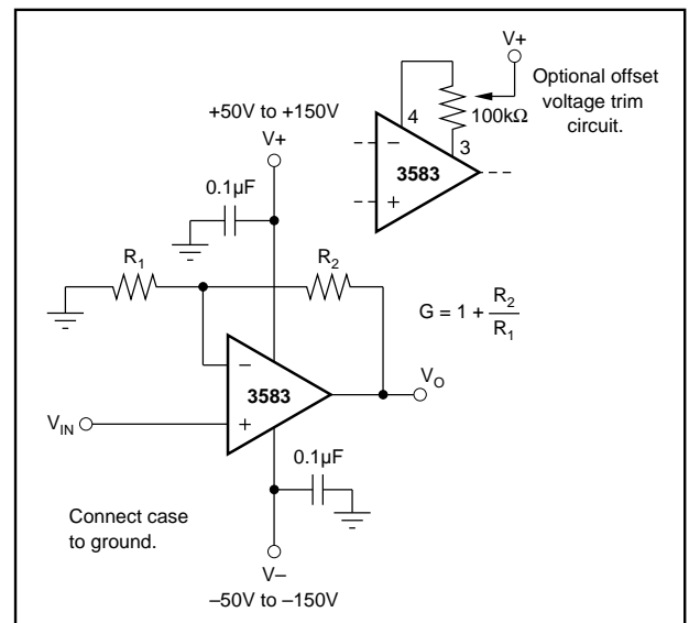
FIGURE 1. Basic Circuit Connections.
