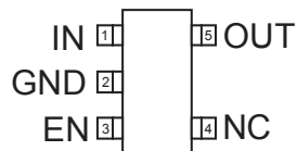
AAT3201 SOT-23-5 (Top View)
