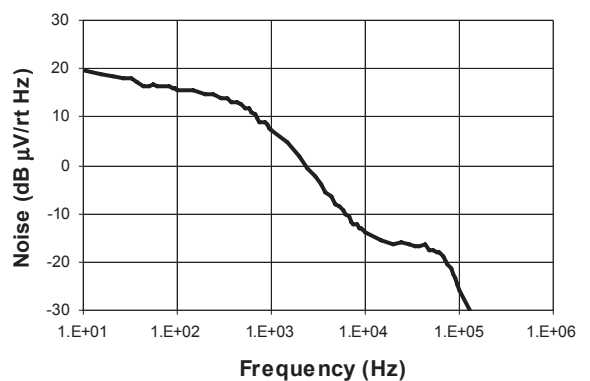
Noise Spectrum
