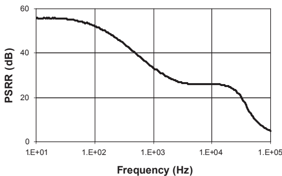
PSRR with 10mA Load
