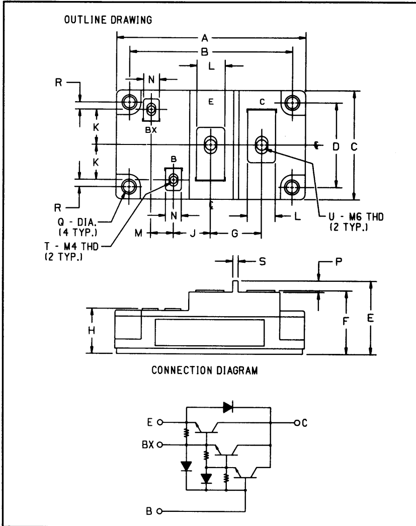
Outline Drawing
