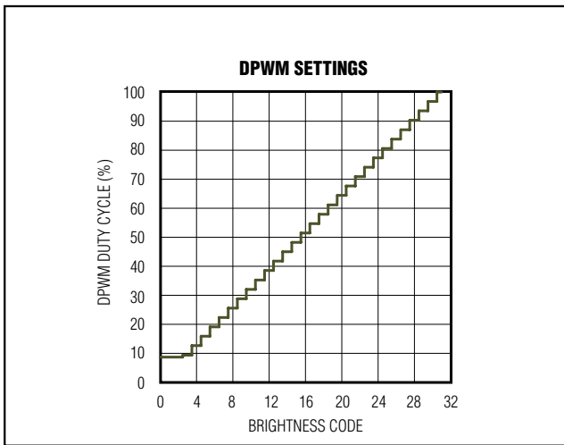
Figure 3. DPWM Settings
