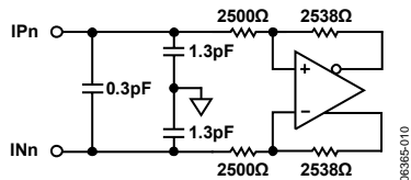
Figure 10. AD8117 Receiver (see also ESD Protection Map, Figure 18)
