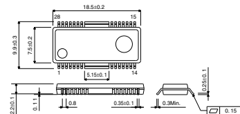
HSOP-M28
