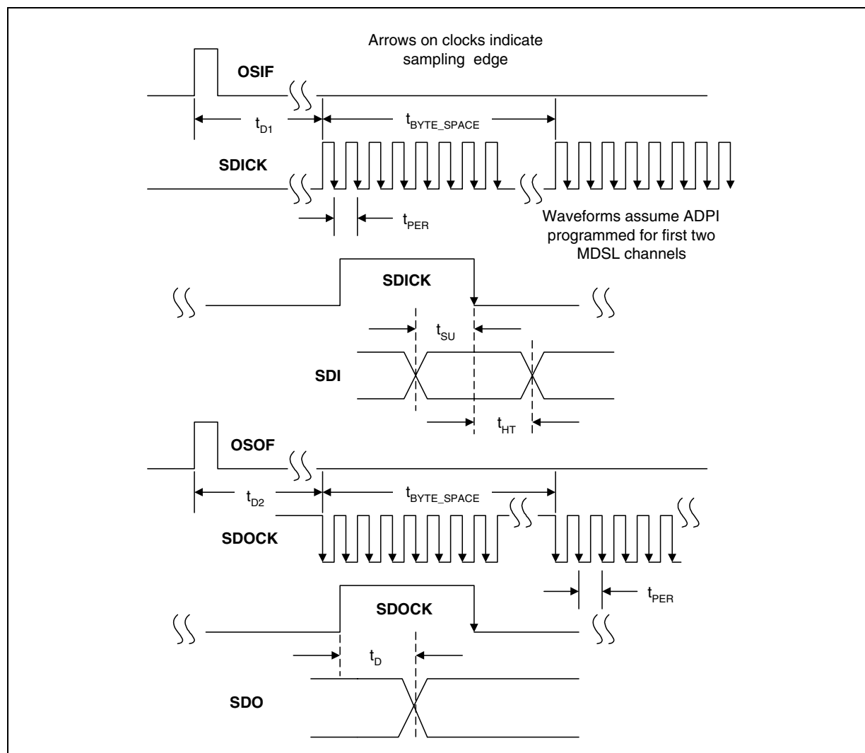
Figure 15. Asynchronous Port Timing
