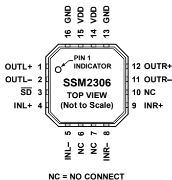
Figure 2. Pin Configuration
