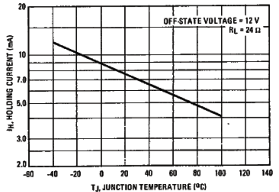
FIGURE 9 -- HOLDING CURRENT
