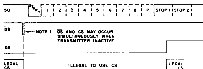
Fig.30 ALLOWABLE POINTS TO USE CONTROL STROBE
