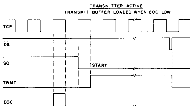
Fig.29 TRANSMITTER AT START BIT
