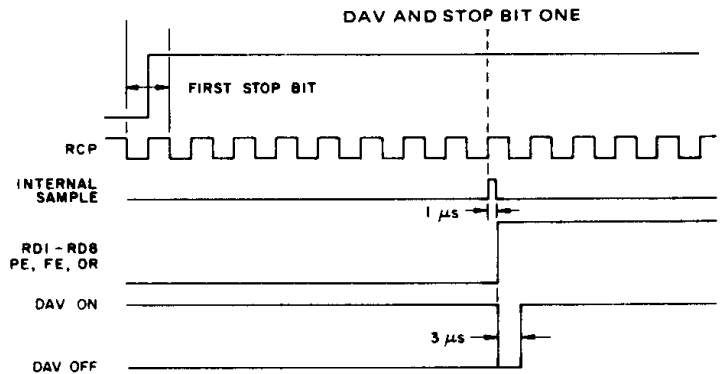
Fig.12 RECEIVER DURING 1st STOP BIT
