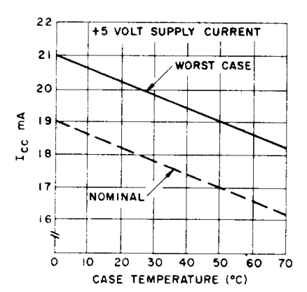
Fig.26 +5 VOLT SUPPLY CURRENT
