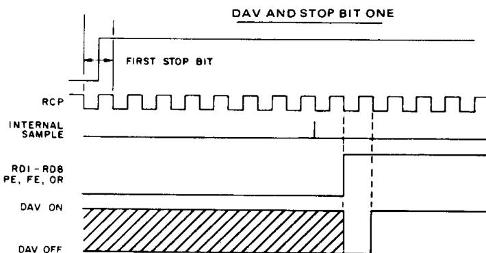
Fig.34 RECEIVER DURING 1ST STOP BIT
