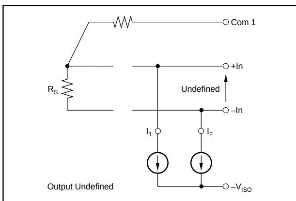
FIGURE 13. -In and +In Open Circuit.
