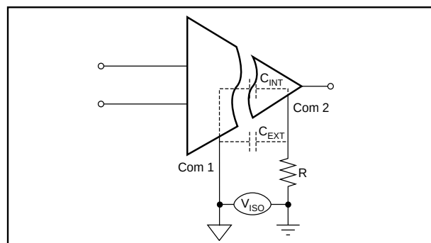
FIGURE 2. Barrier Capacitance.
