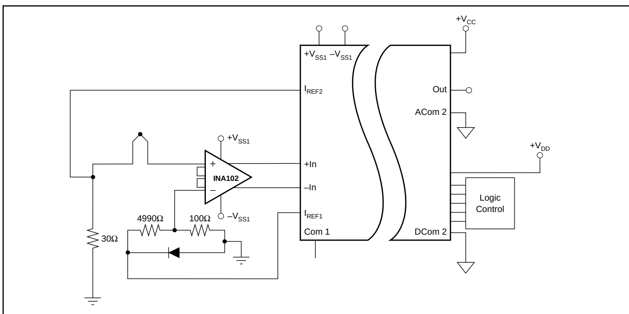
FIGURE 19. Thermocouple with Cold Junction Compensation.
