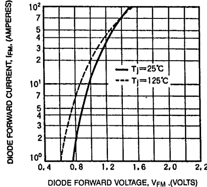
DIODE CHARACTERISTICS (TYPICAL)
