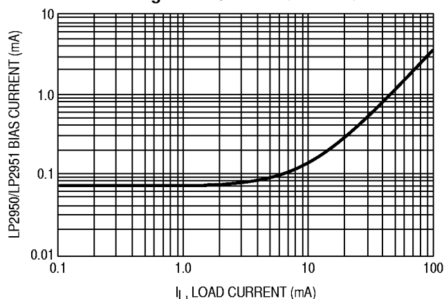
Figure 1. Quiescent Current
