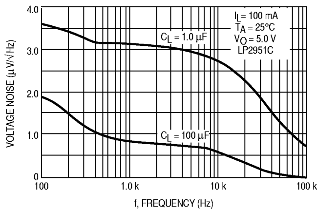
Figure 12. Output Noise
