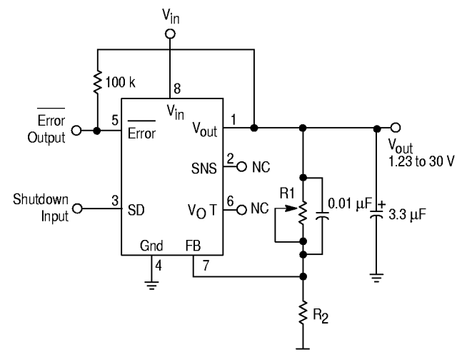
Figure 16. Adjustable Regulator
