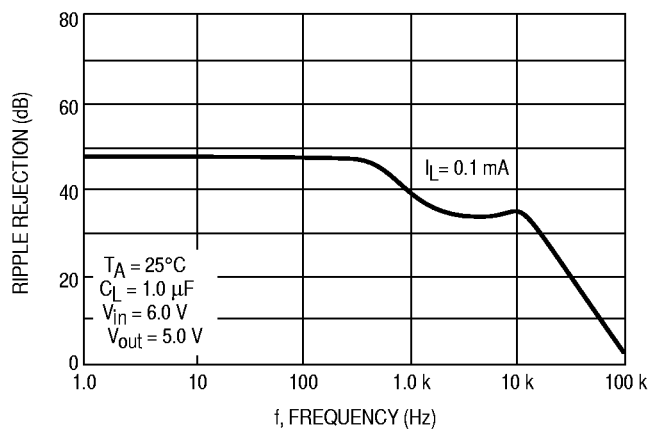
Figure 11. Ripple Rejection
