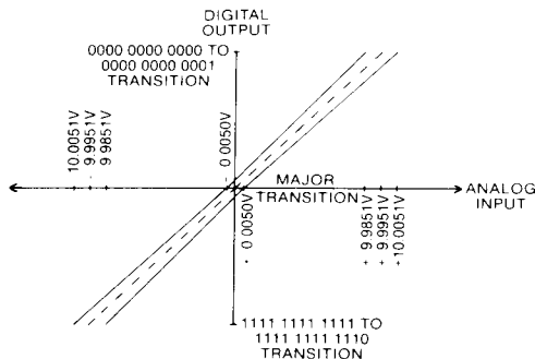
MN5212 ABSOLUTE ACCURACY +25^\circ \text{C}
