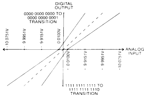
MN5212H ABSOLUTE ACCURACY -55^\circ \text{C} AND +125^\circ \text{C}
