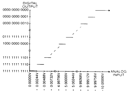
MN5216 TRANSFER FUNCTION
