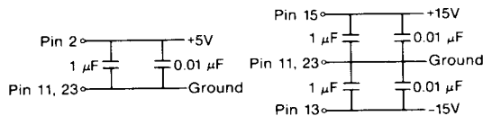
POWER SUPPLY DECOUPLING
