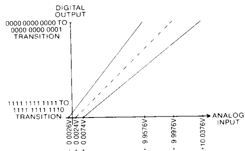
MN5216H ABSOLUTE ACCURACY -55°C AND +125°C
