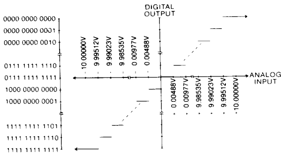
MN5212 TRANSFER FUNCTION
