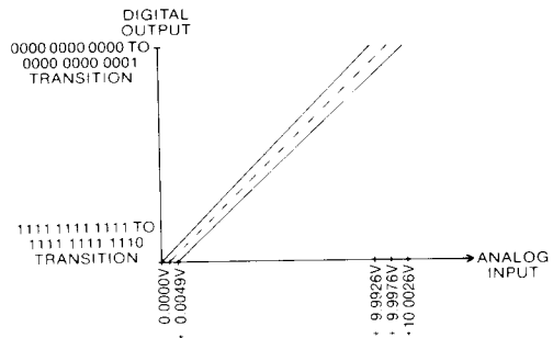
MN5216 ABSOLUTE ACCURACY +25°C
