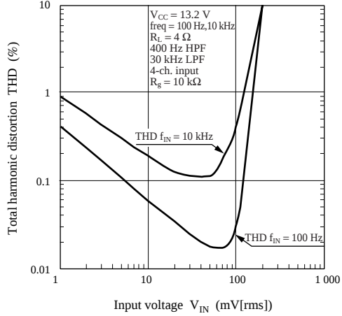
THD — V_{IN}
