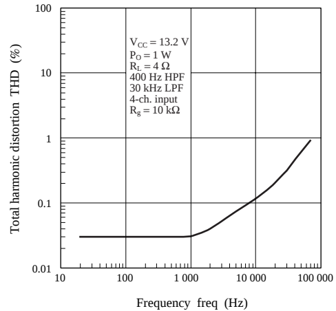
THD — freq
