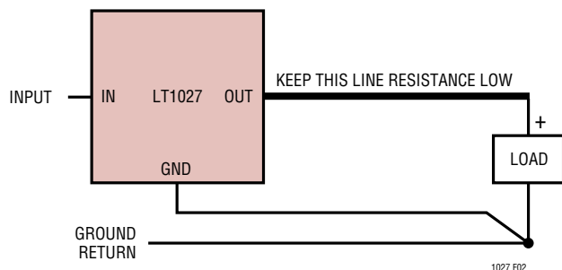
Figure 2. Standard Hook-Up
