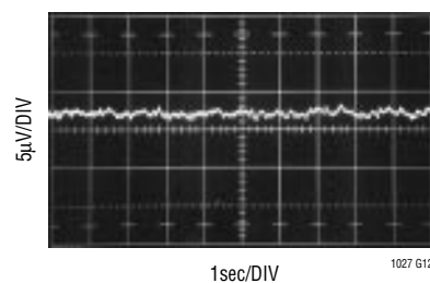
0.1Hz to 10Hz Output Noise Filtering = 1 zero at 0.1Hz 2 poles at 10Hz
