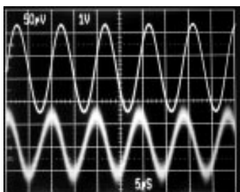
REFERENCE FEEDTHROUGH AT 100kHz
