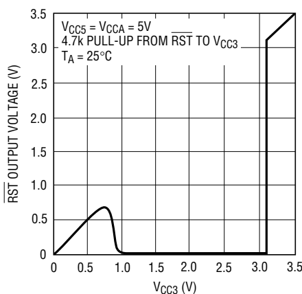
\overline{RST} Output Voltage vs Supply Voltage
