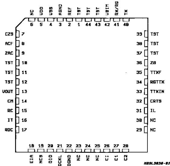
PLCC44
