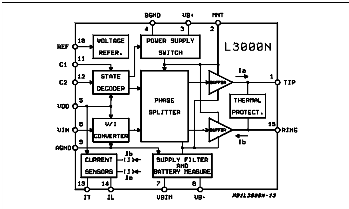
L3000N BLOCK DIAGRAM
