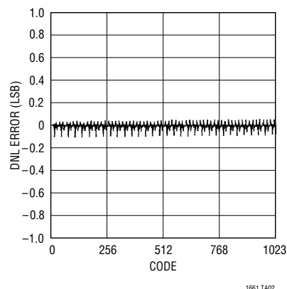
Differential Nonlinearity (DNL)
