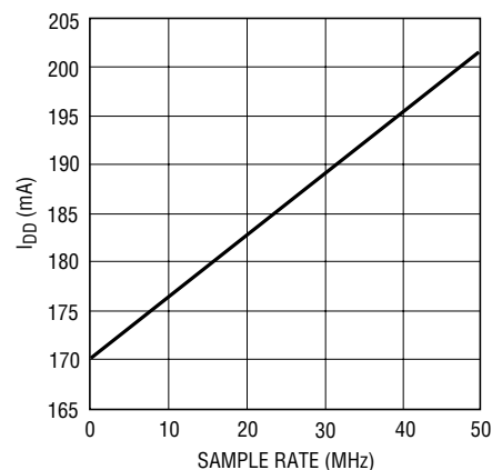
I DD vs Sample Rate
