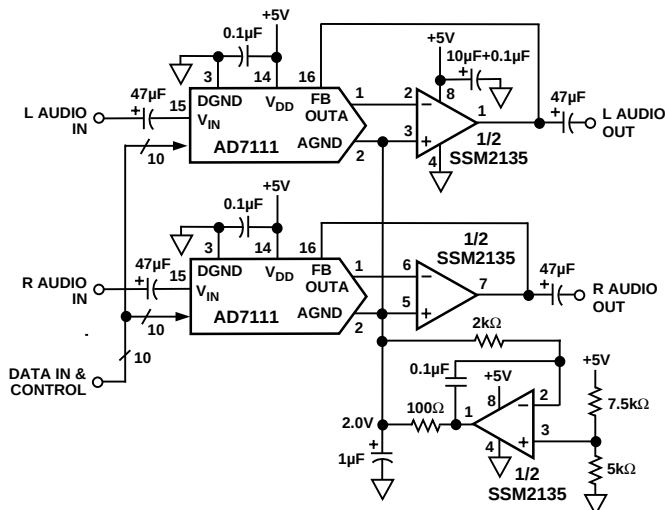
Figure 38. Single Supply Logarithmic Volume Control
