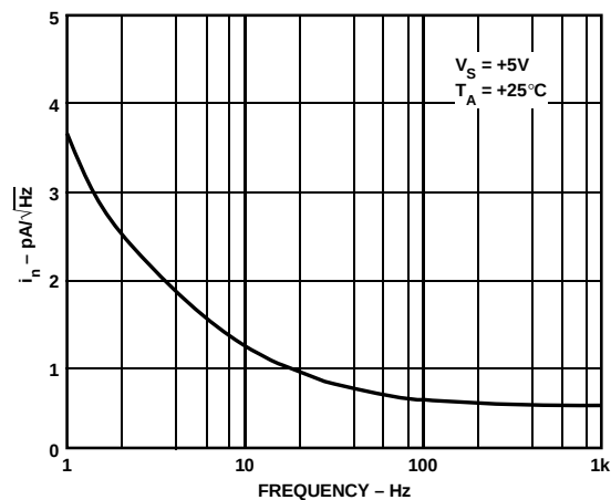
Figure 10. Current Noise Density vs. Frequency
