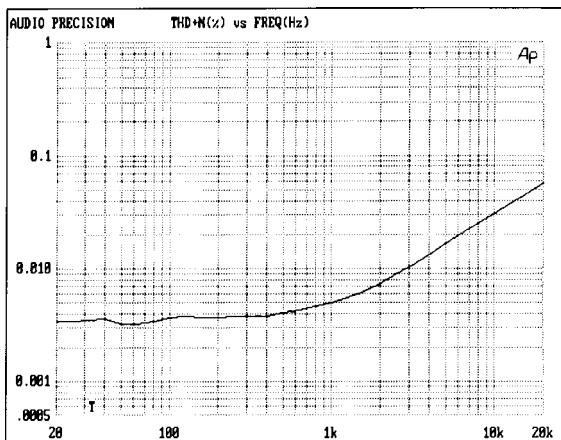
Figure 30. Headphone Driver THD+N vs. Frequency into a 32\ \Omega Load ( V_S = +5\text{ V} , with 80\text{ kHz} Low-Pass Filter)
