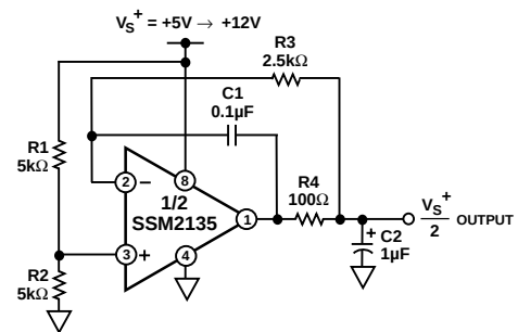
Figure 36. Pseudo-Reference Generator
