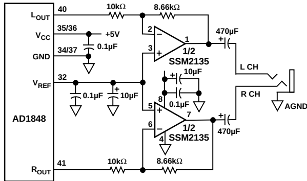
Figure 29. A Stereo Headphone Driver for Multimedia Sound Codec
