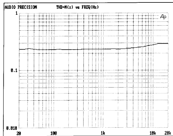
Figure 32. MIC Preamp THD+N Performance ( V_S = +5\text{ V} , A_V = 40\text{ dB} , V_{\text{OUT}} = 1\text{ V rms} , with 80\text{ kHz} Low-Pass Filter)
