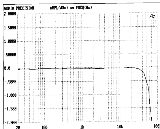
Figure 11. Frequency Response ( A_V = +1 , V_S = +5 V, V_{IN} = 1 V p-p, R_L = 10 k \Omega )
