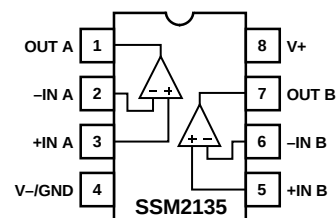
8-Lead Epoxy DIP (P-Suffix)
