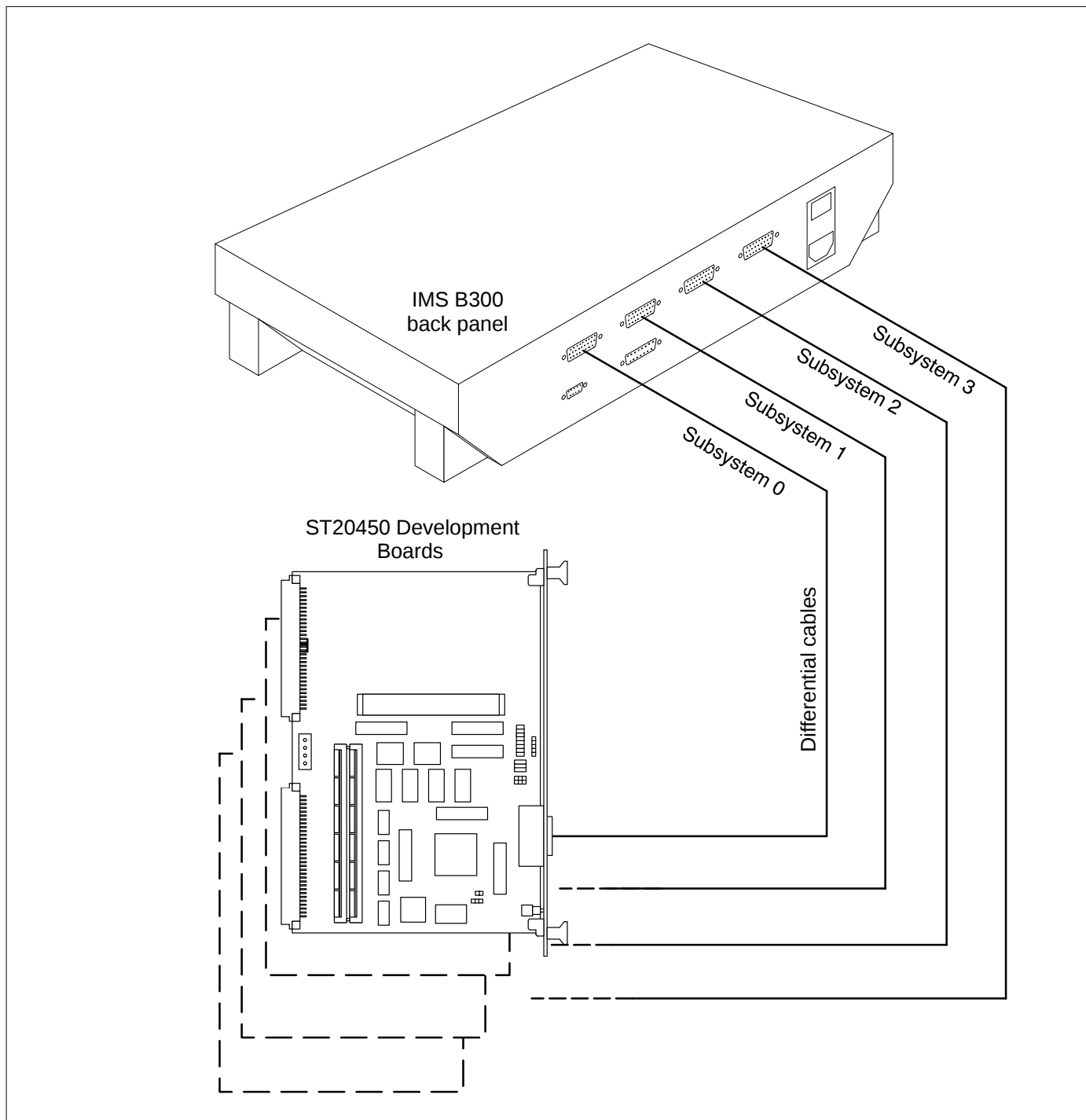
Figure 3 Connection of four IMS B300 differential cables to ST20450 Development Boards
