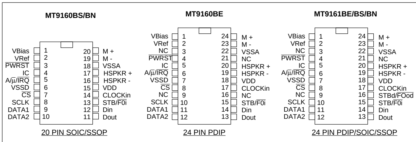
Figure 2 - Pin Connections
