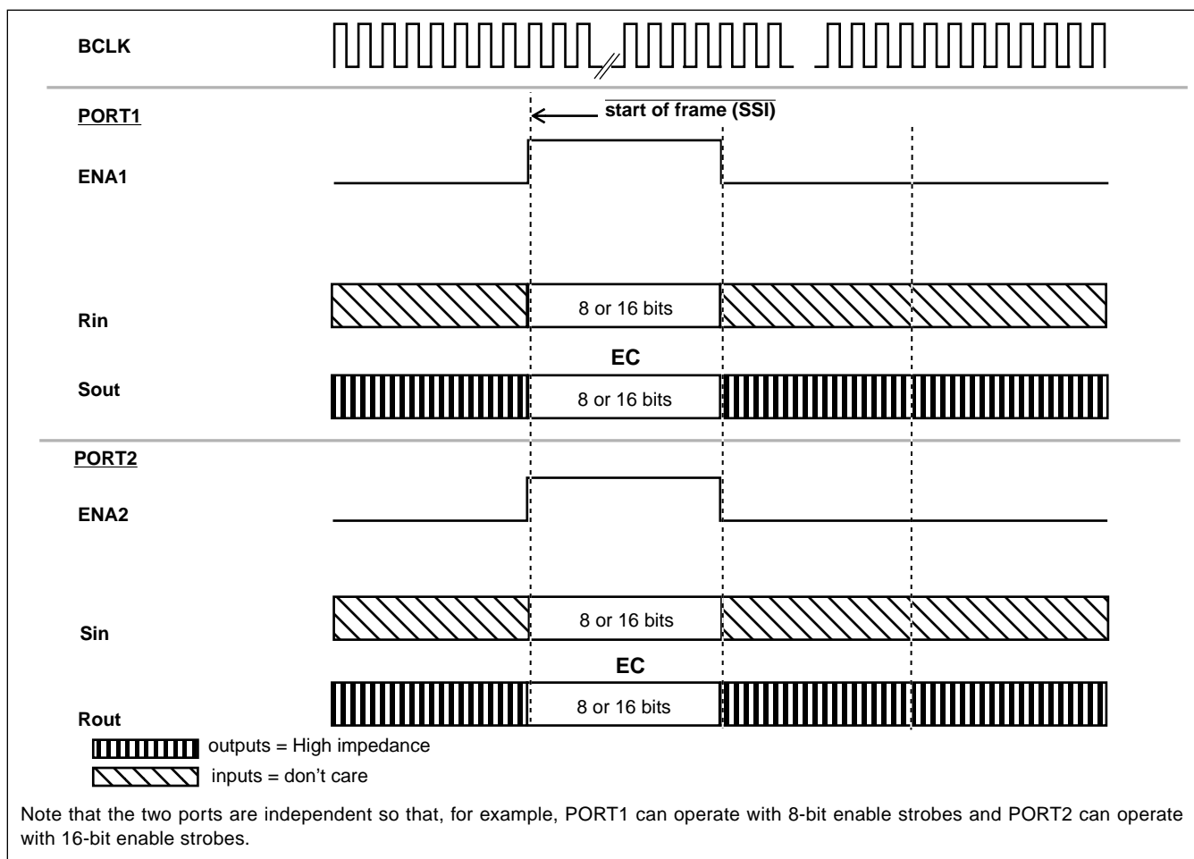
Figure 7 - SSI Operation
