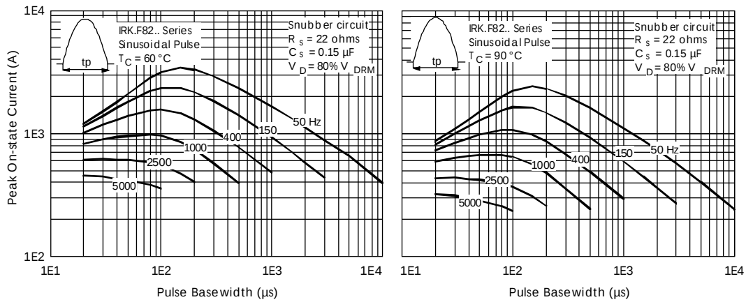
Fig. 11 - Frequency Characteristics
