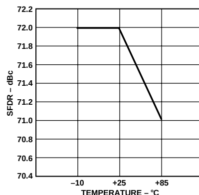
Figure 4. SFDR vs. Temperature @ f_{CLOCK} = 50\text{ MHz} ( f_{OUT} = 1\text{ MHz} )
