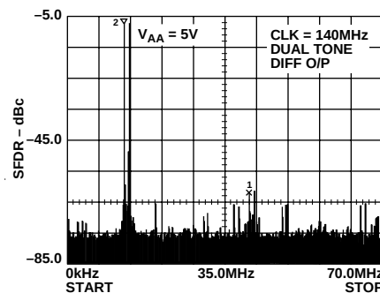
Figure 10. Dual-Tone SFDR @ f_{CLOCK} = 140\text{ MHz} ( f_{OUT1} = 13.5\text{ MHz} , f_{OUT2} = 14.5\text{ MHz} )
