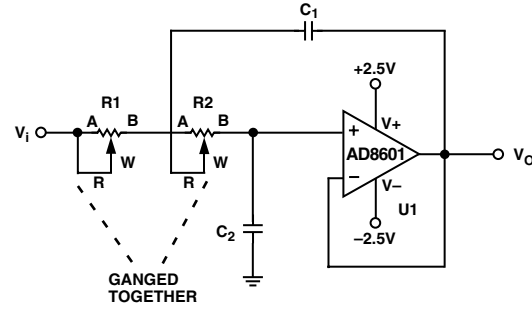
Figure 17. Sallen Key Low-Pass Filter
