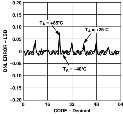
TPC 2. DNL vs. Code, T_A = -40^\circ\text{C} , +25^\circ\text{C} , +85^\circ\text{C} Overlay, R_{AB} = 10\text{ k}\Omega
