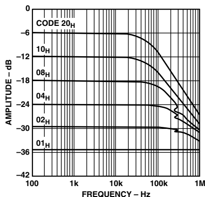
TPC 14. Gain vs. Frequency vs. Code, R_{AB} = 100 \text{ k}\Omega . Test Circuit 7.
