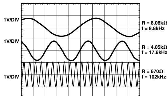
Figure 22. Programmable Oscillation
