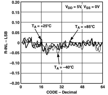
TPC 3. R-INL vs. Code, T_A = -40^\circ\text{C} , +25^\circ\text{C} , +85^\circ\text{C} Overlay, R_{AB} = 10\text{ k}\Omega
