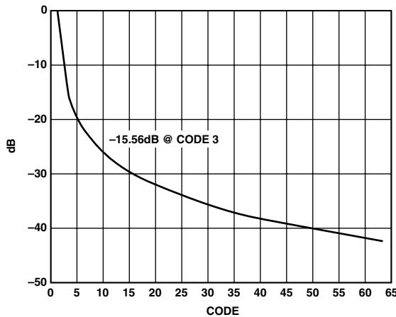
Figure 8. Plot of Log_Error Conformance for Odd Numbers of Bits Only (Even Numbers of Bits is Ideal)
