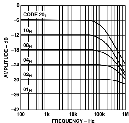
TPC 13. Gain vs. Frequency vs. Code, R_{AB} = 50 \text{ k}\Omega . Test Circuit 7.
