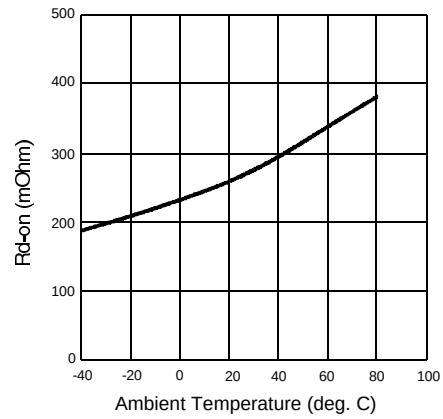
Figure 4. Typical On-Resistance
