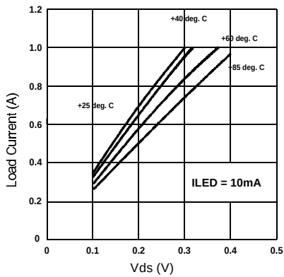
Figure 3. Typical On-Characteristics
