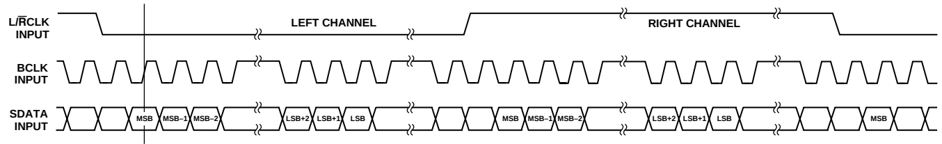
Figure 2. I²S-Justified Mode
