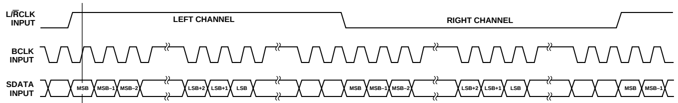
Figure 3. Left-Justified Mode
