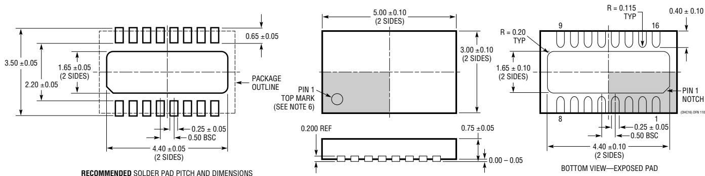
DHC Package 16-Lead Plastic DFN (5mm × 3mm) (Reference LTC DWG # 05-08-1706)
