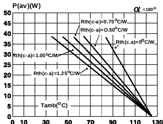
Fig.4 : Correlation between maximum average power dissipation and maximum allowable temperature (Tamb) for different thermal resistances heatsink + contact. (Rectangular waveform : Thyristor or Diode)
