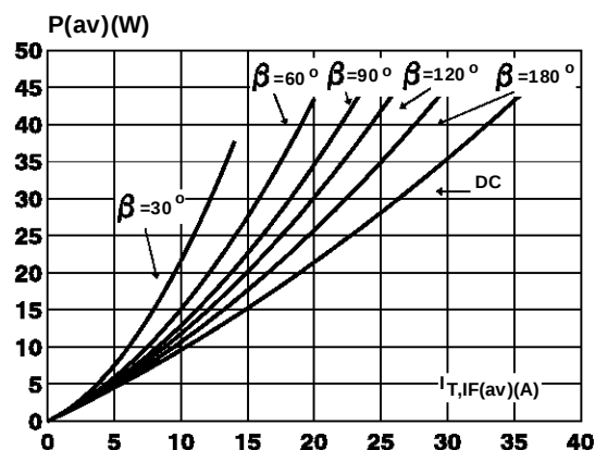
Fig.5 : Maximum total power dissipation versus output current on resistive or inductive load. (Single phase bridge rectifier : 2 packages MDS35)
