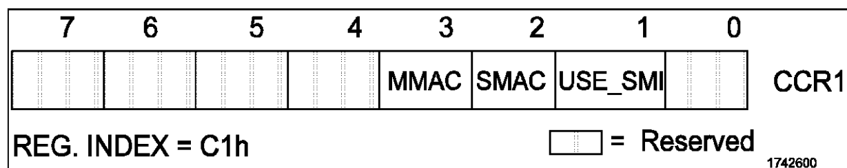
Figure 1.3. Configuration Control Register 1 (CCR1)
