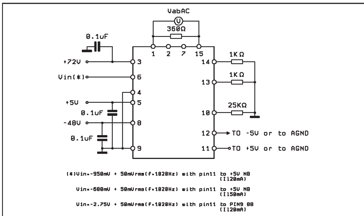
Figure 5: Receiving Gain
