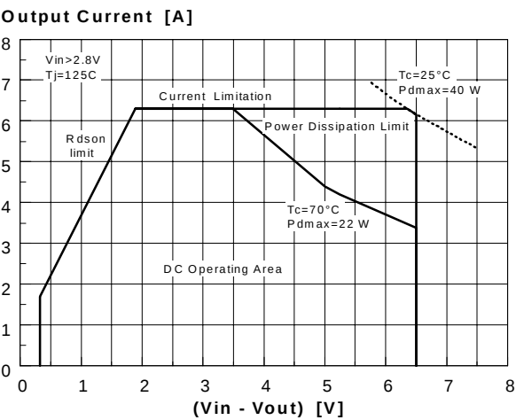
Figure 4: DC Operating Area
