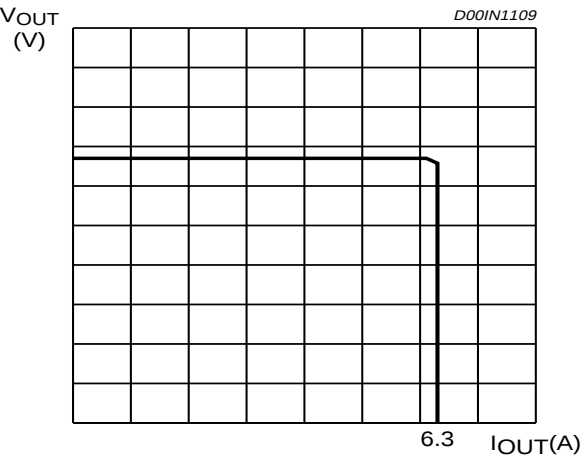
Figure 6: Output Voltage vs. Output Current. (VOUT = 1.5V)
